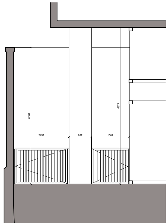
A - River Walk gate Elevation 1:100
