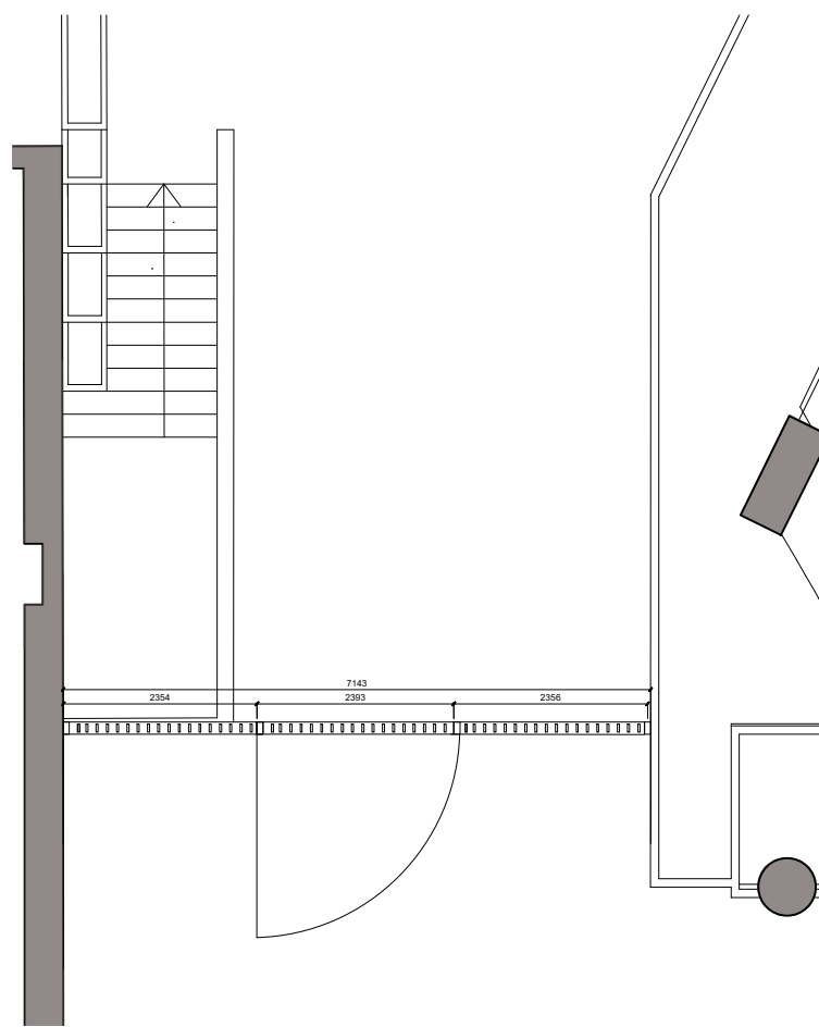
C - River Building gate Plan 1:100
