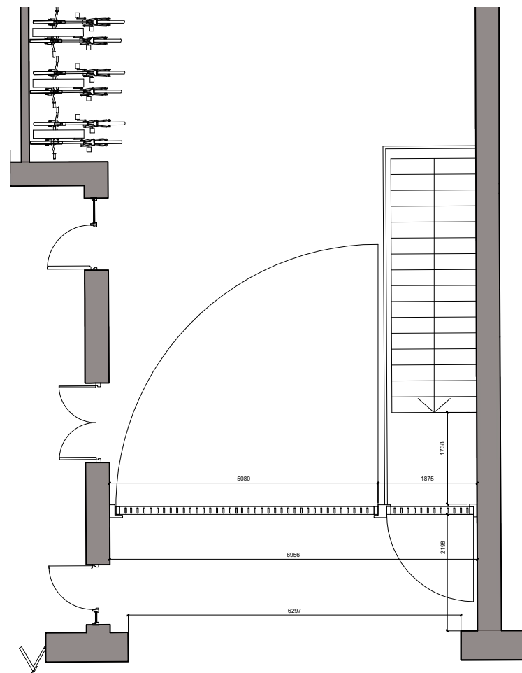
B - Block B gate Plan 1:100
