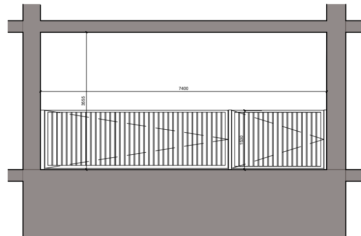
B - Block B gate Elevation 1:100
