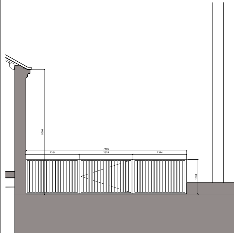
C - River Building gate Elevation 1:100
