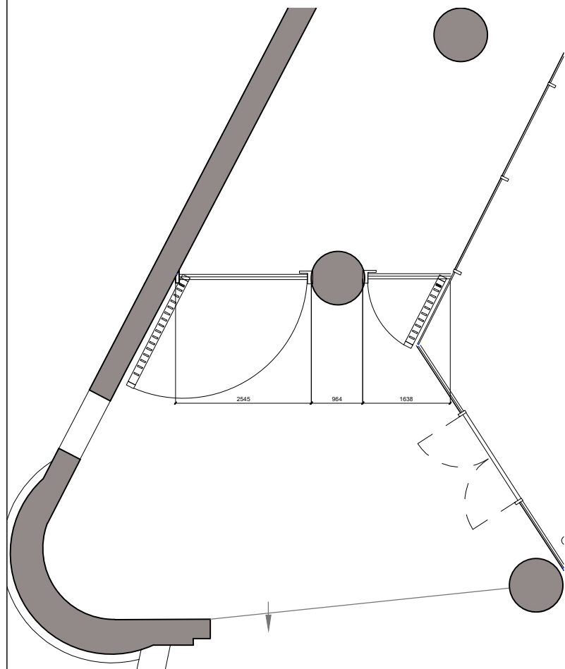
A - River Walk gate Plan 1:100
